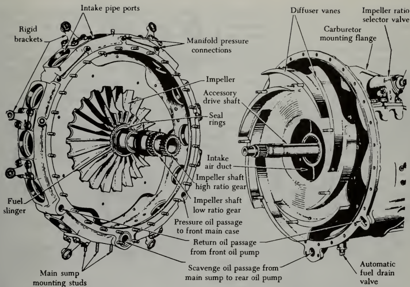
FIGURE 2-8. Blower and intermediate rear sections.
